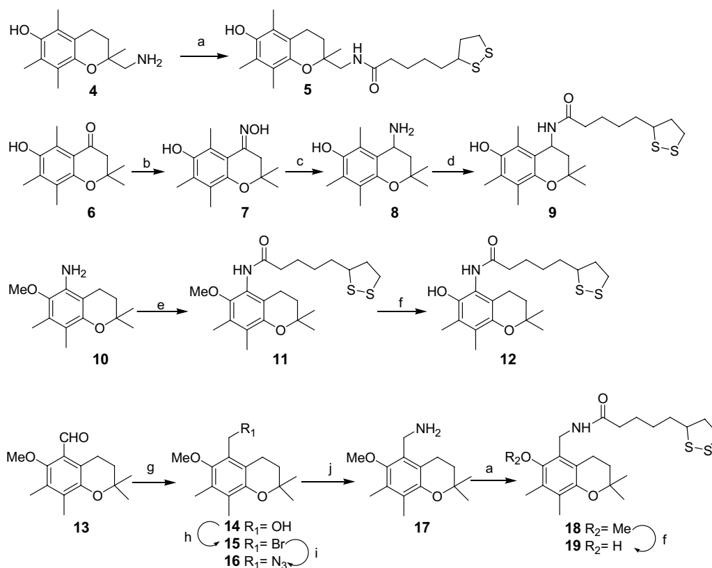
Scheme 2. Reagents and conditions: (a) N -hydroxysuccinimide-activated lipoic acid; (b) \text{NH}_2\text{OH}\cdot\text{HCl} , pyridine; (c) \text{TiCl}_4 , \text{NaBH}_4 , DME; (d) lipoic acid chloride, \text{NaHCO}_3 , THF, \text{H}_2\text{O} ; (e) lipoic acid chloride, \text{Et}_3\text{N} , THF; (f) \text{BF}_3\cdot\text{S}(\text{Me})_2 , \text{CH}_2\text{Cl}_2 ; (g) \text{NaBH}_3\text{CN} , AcOH, acetonitrile; (h) \text{PBr}_3 , \text{CH}_2\text{Cl}_2 ; (i) \text{NaN}_3 , DMF; (j) \text{PPh}_3 , THF, \text{H}_2\text{O} .
