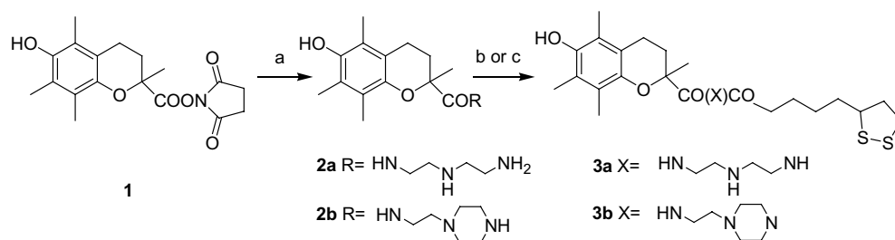
Scheme 1. Reagents and conditions: (a) diethylenetriamine or 1-(2-aminoethyl)piperazine; (b) N -hydroxysuccinimide-activated lipoic acid; (c) lipoic acid chloride, NaHCO 3 , THF, H 2 O.
